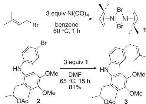
Scheme 1. A rare example of selective prenylation of aryl halide.
