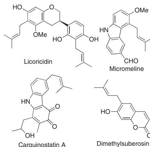
Figure 1. Some natural products bearing prenyl groups.
