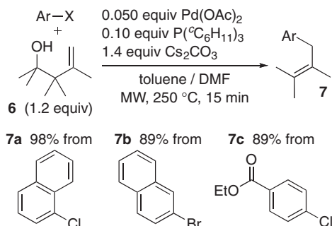
Scheme 3. Synthesis of 2,3-dimethyl-2-butenylarenes.
