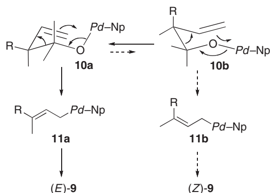
Scheme 4. Origin of stereoselectivity.
